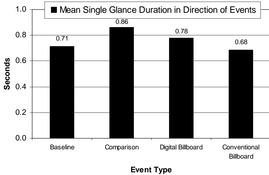
Figure 30. Mean Glance Time for Glances in the Direction of an Event for the Nighttime Exploratory Study.
