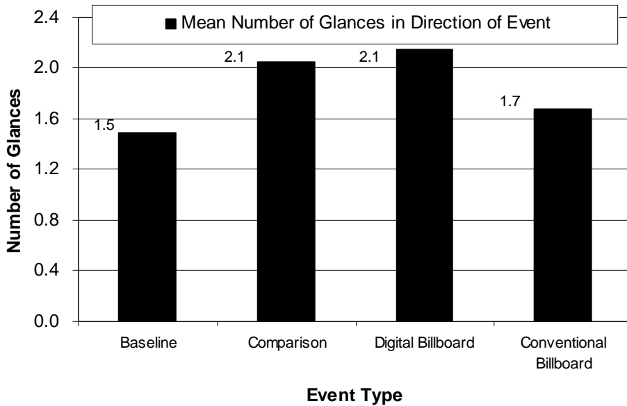
Figure 31. Mean Number of Glances in the Direction of an Event for the Nighttime Exploratory Study.
