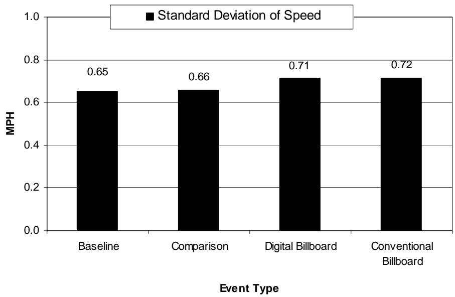
Figure 26. Standard Deviation of Speed by Event for Events Occurring on Interstates, in miles per hour. (None of the observed differences was significant.)
