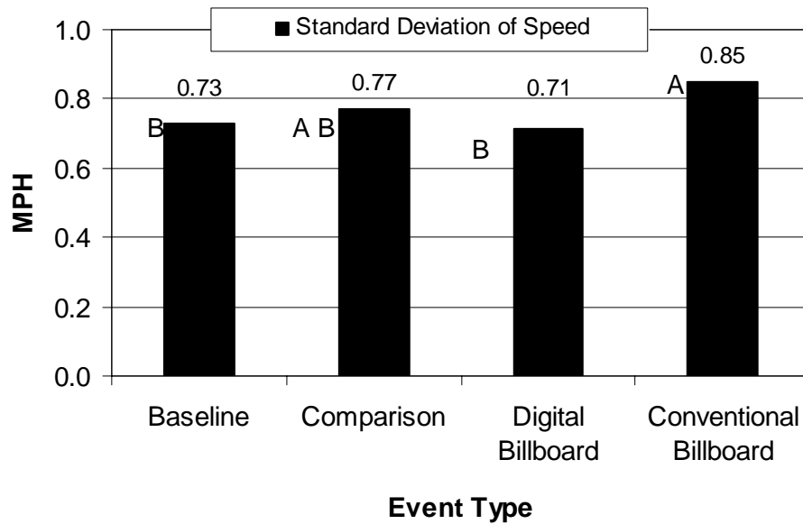
Figure 25. Standard Deviation of Speed by Event, in miles per hour. (Data points with a shared letter do not differ significantly from one another.)
